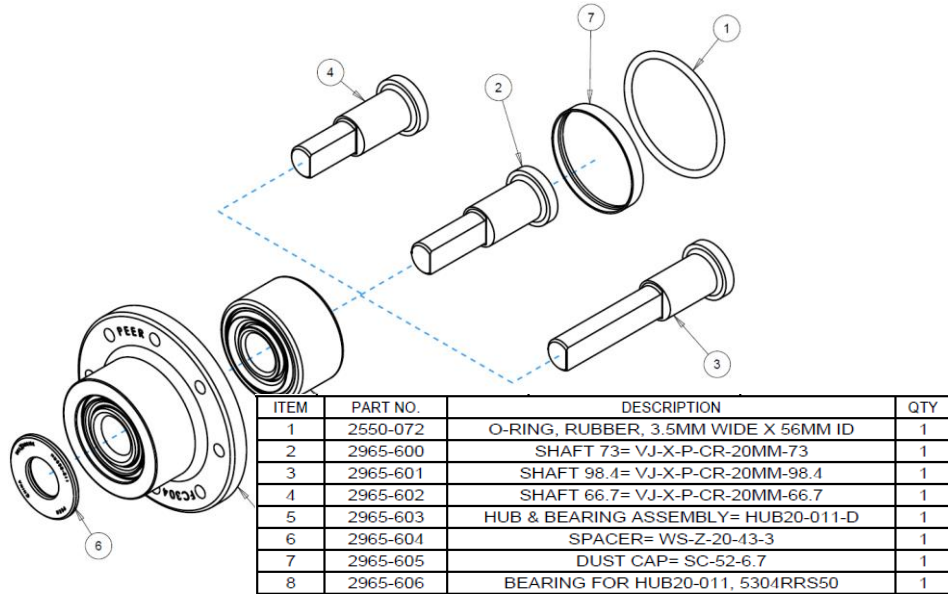
8 BOLT HUB
