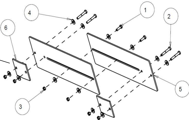
2940-084 UNIVERSAL HAND RAIL MOUNT KIT
