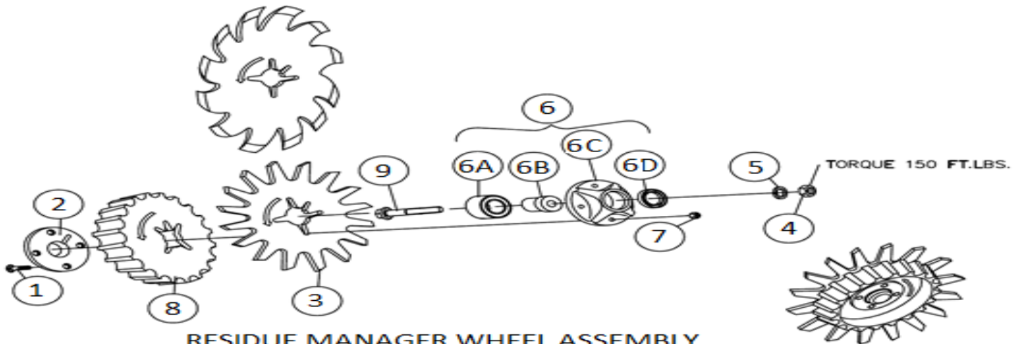
RESIDUE MANAGER WHEEL ASSEMBLY (1 WHEEL ASSEMBLY)
