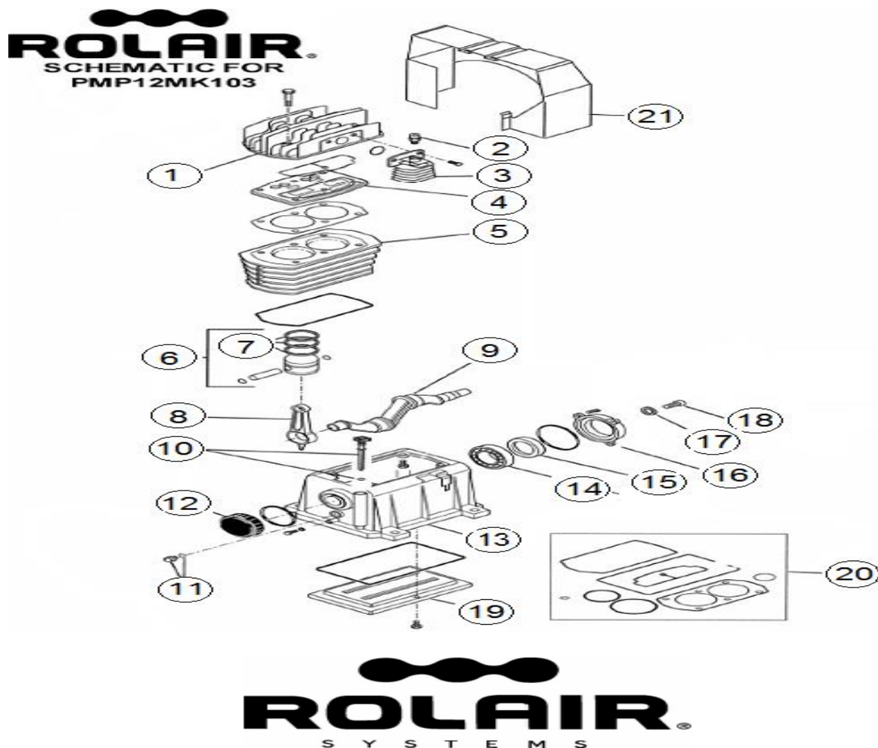
PARTS LIST FOR PMP12MK103
