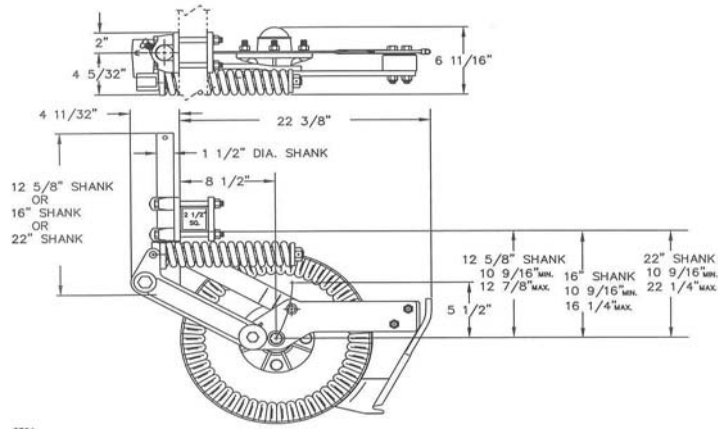
YETTER MODEL 2995 LIQUID FERTILIZER COULTER
