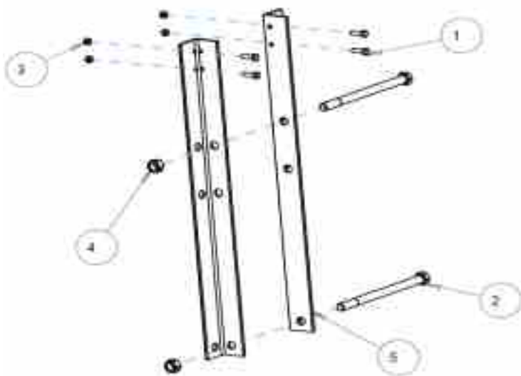
2940-083 8X16 & 8X12 BAR MOUNT KIT
