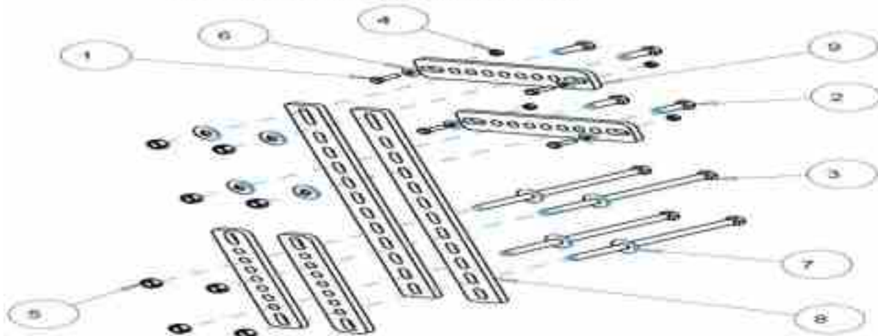
2940-082 5X7 & 7X7 BAR MOUNT KIT
