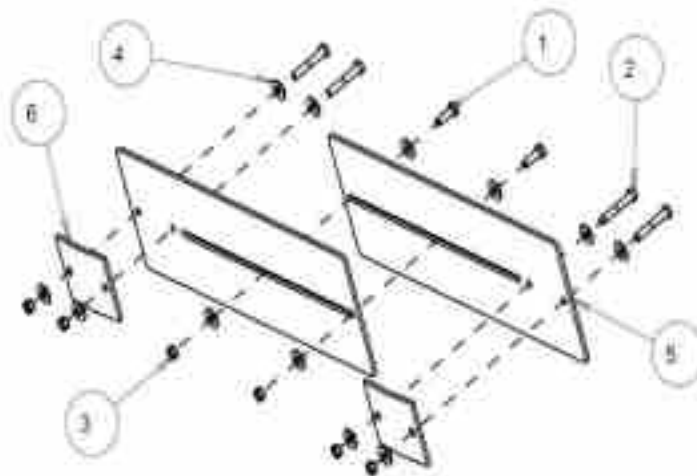
2940-084 UNIVERSAL HAND RAIL MOUNT KIT
