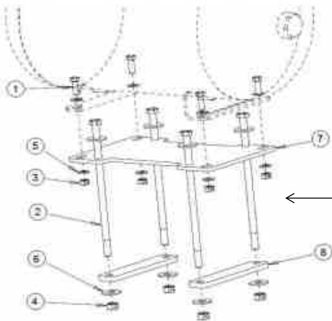
2940-090 8x12 & 2940-091 8x16 HYD COMP MOUNT KIT
